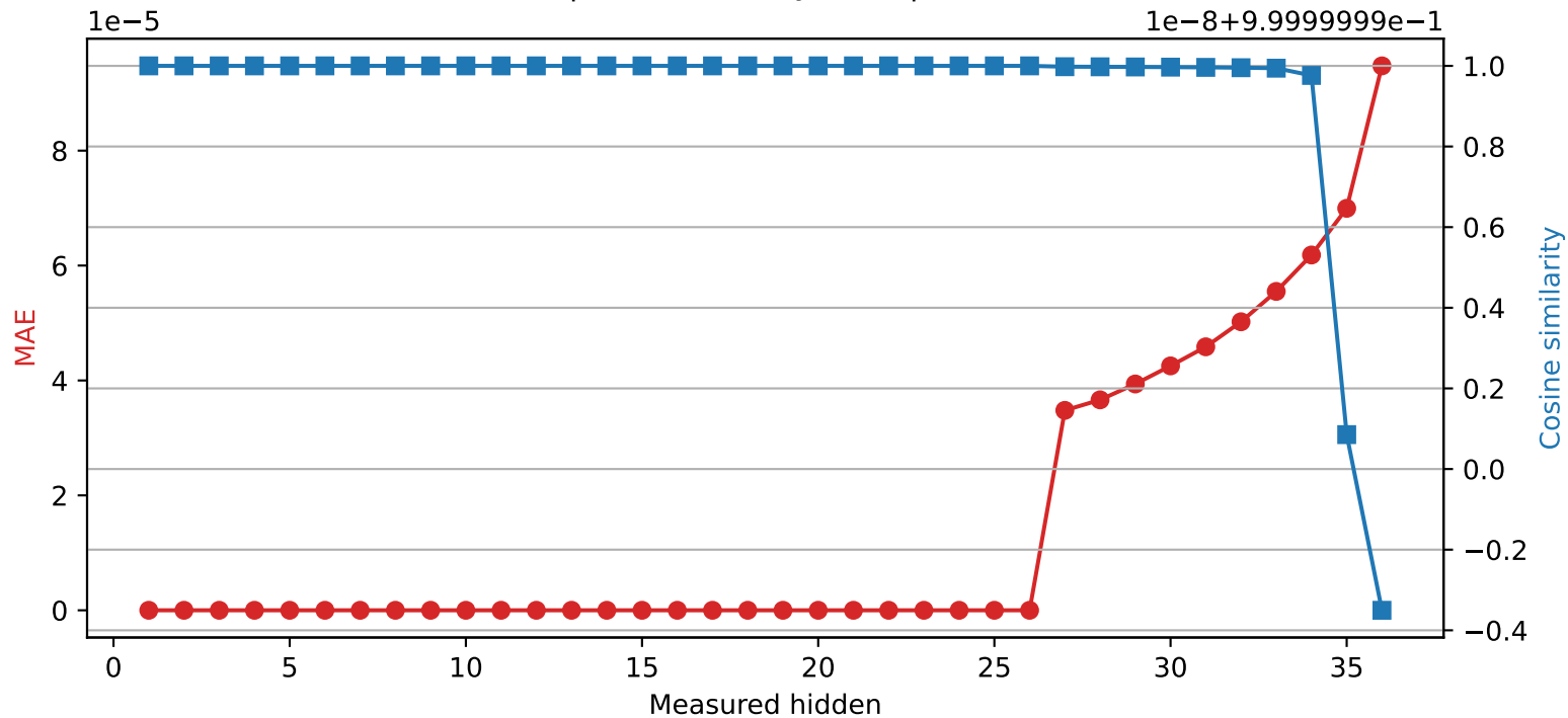
SmolLM3-3B | Quantized layer 26 | float32 → int16
