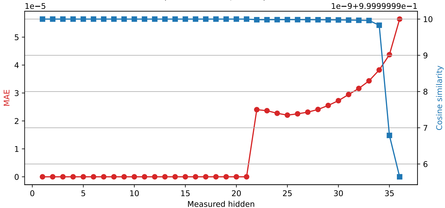
SmolLM3-3B | Quantized layer 21 | float32 → int16
