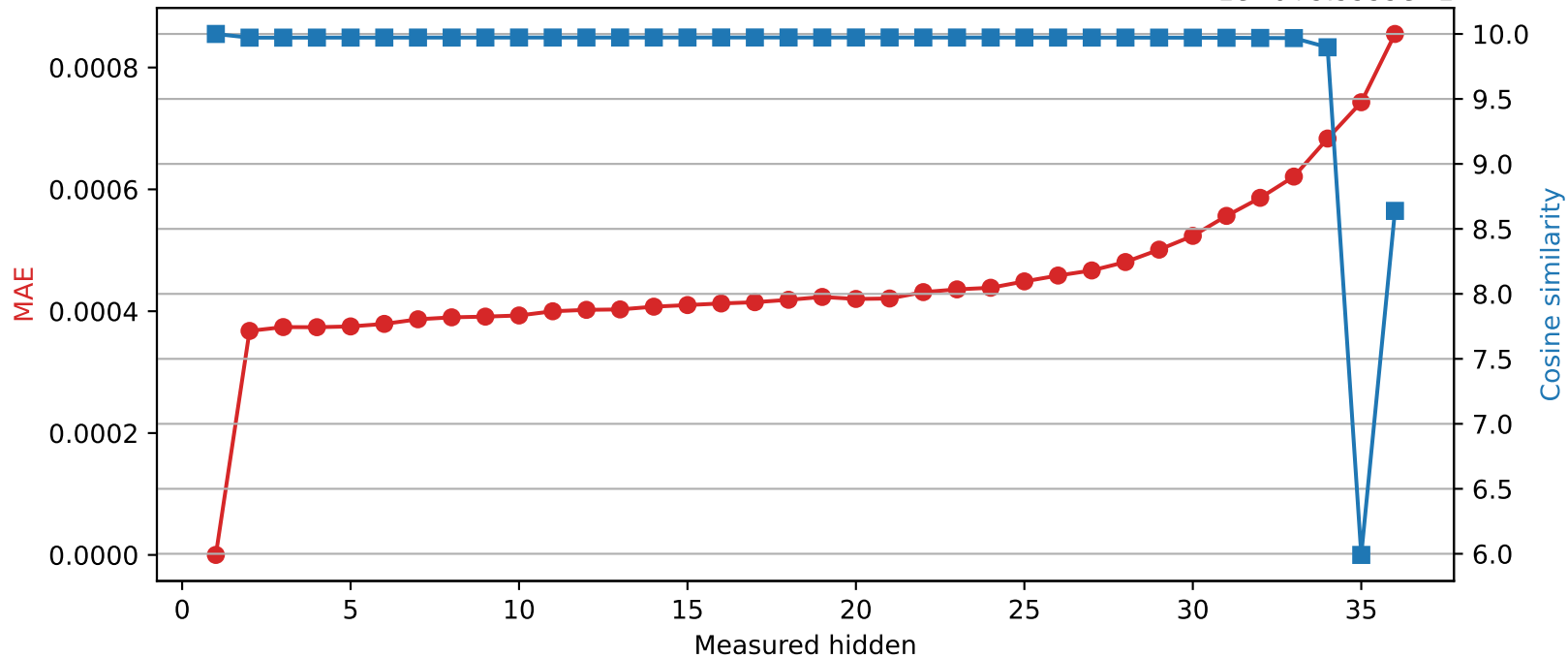
SmolLM3-3B | Quantized layer 1 | float32 → int16 1e-6+9.9999e-1
