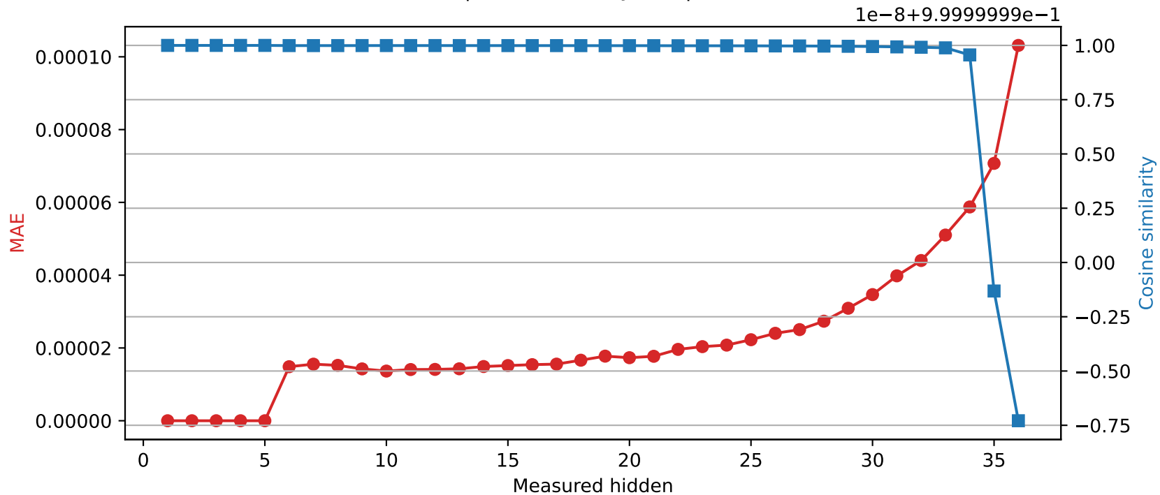
SmolLM3-3B | Quantized layer 5 | float32 → int16
