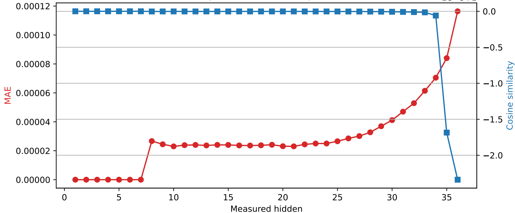
SmolLM3-3B | Quantized layer 7 | float32 → int16
