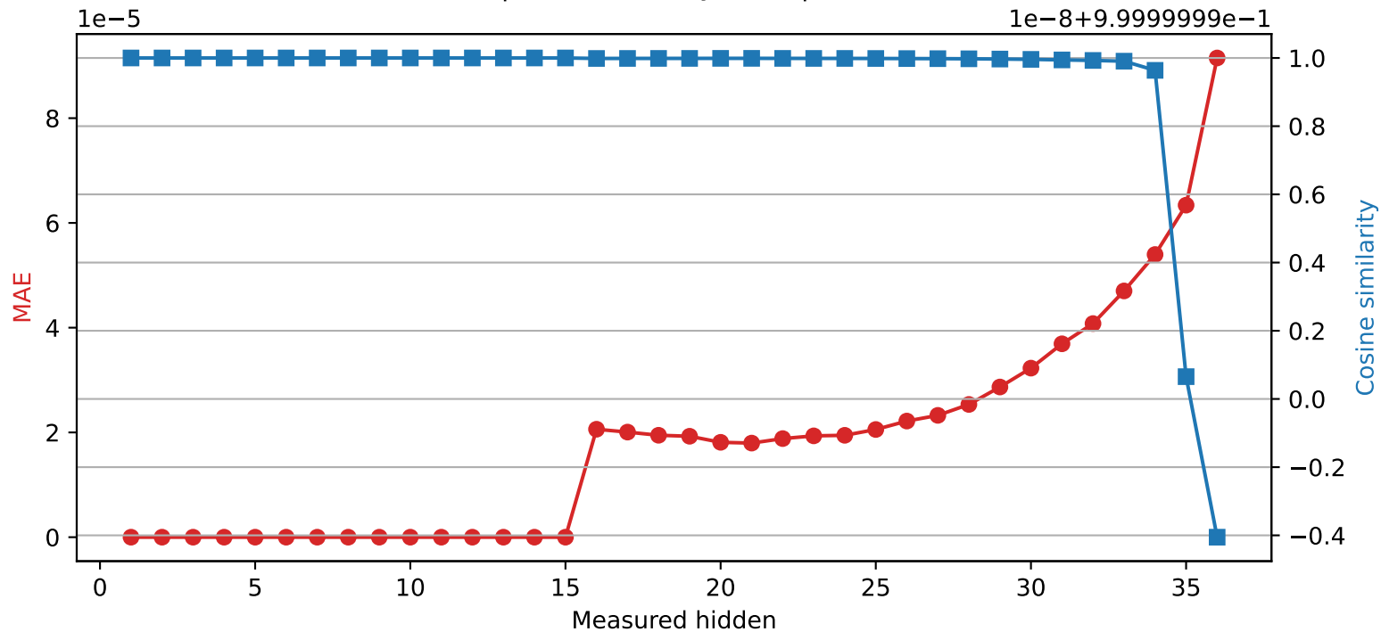
SmolLM3-3B | Quantized layer 15 | float32 → int16
