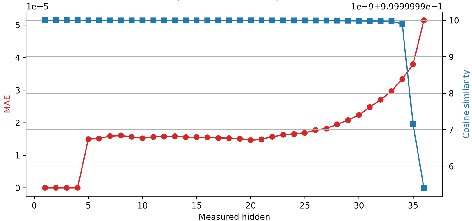
SmolLM3-3B | Quantized layer 4 | float32 → int16
