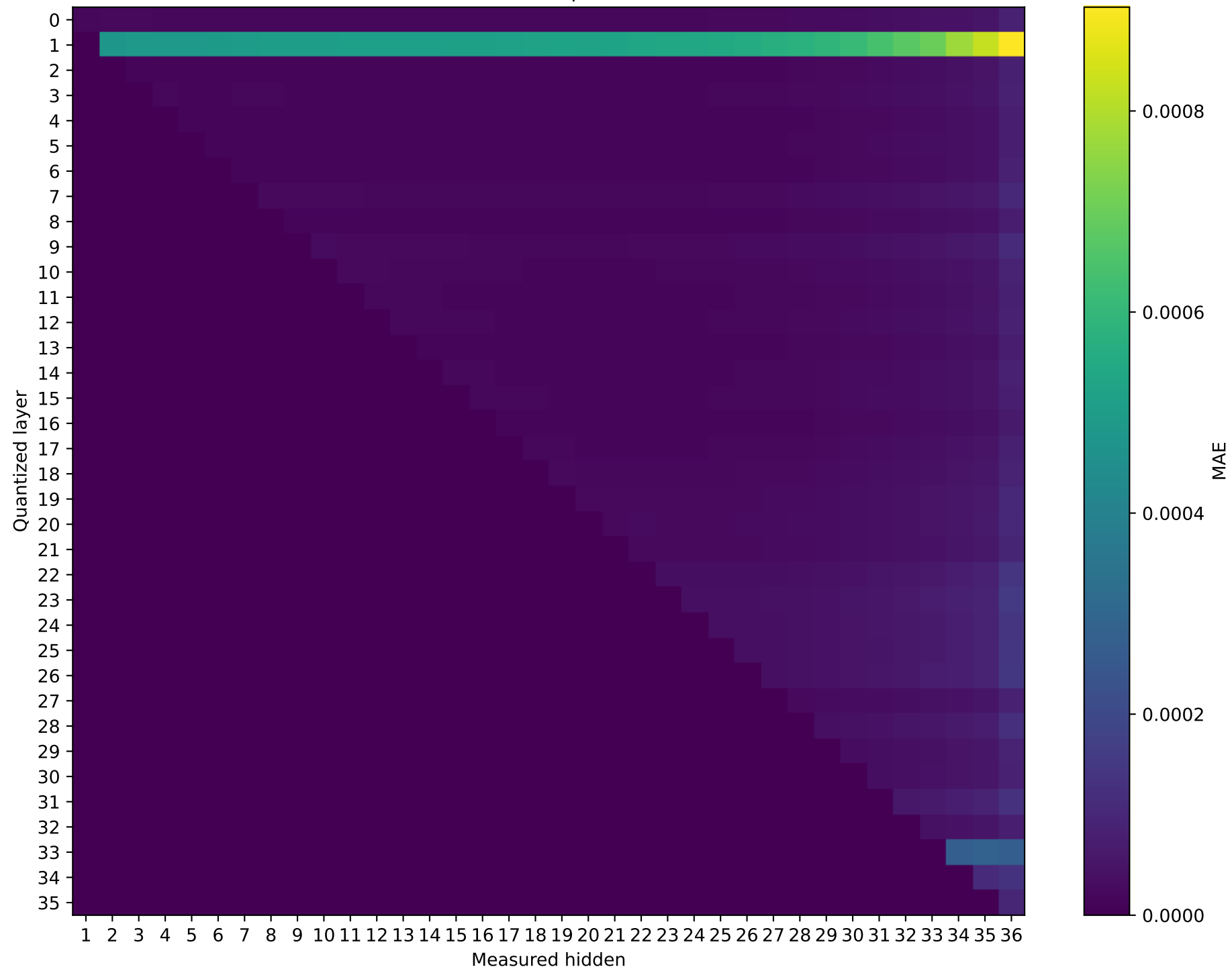
Model: SmolLM3-3B | float64 → int16
