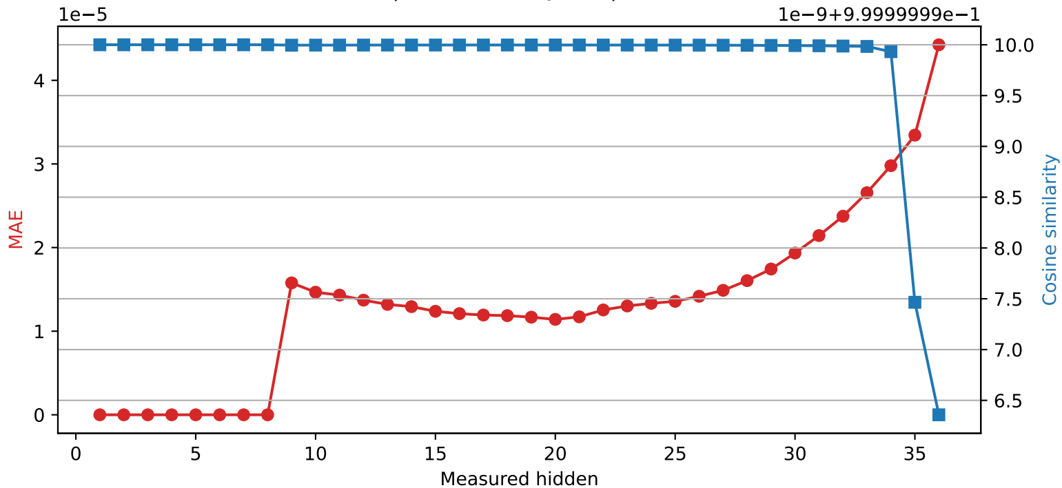
SmolLM3-3B | Quantized layer 8 | float64 → int16
