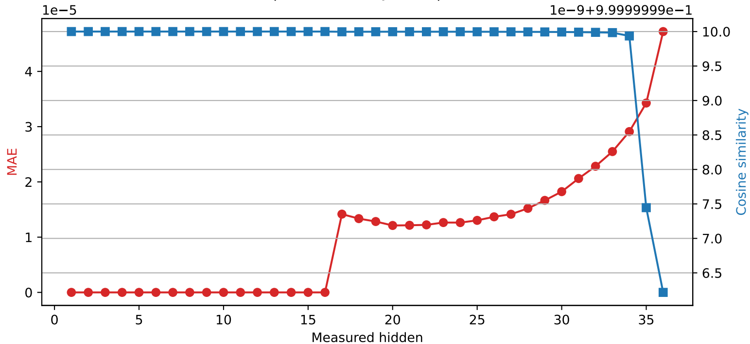
SmolLM3-3B | Quantized layer 16 | float64 → int16
