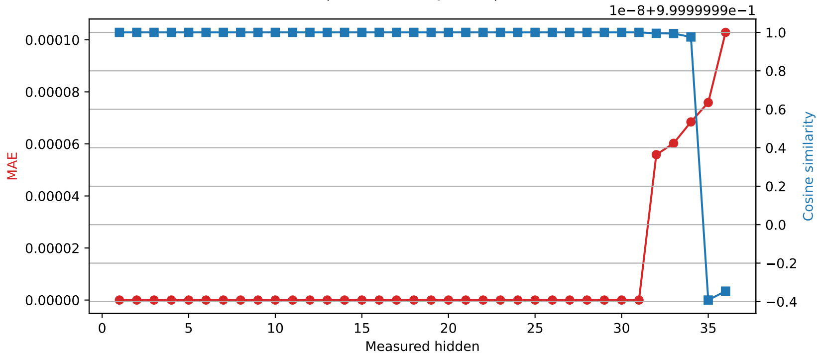
SmolLM3-3B | Quantized layer 31 | float64 → int16
