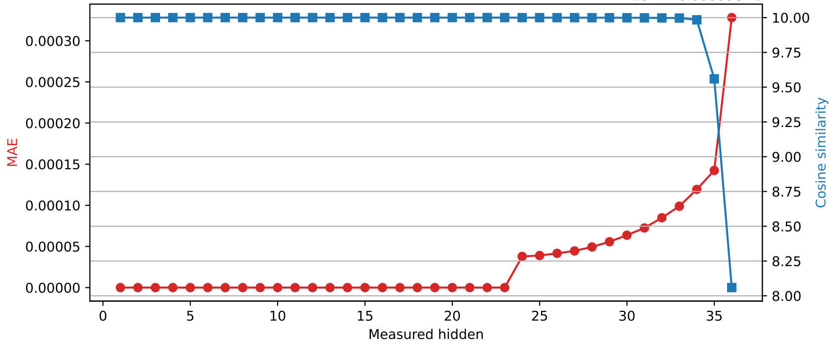
SmolLM3-3B | Quantized layer 23 | float64 \rightarrow int16 1e-7+9.99999e-1
