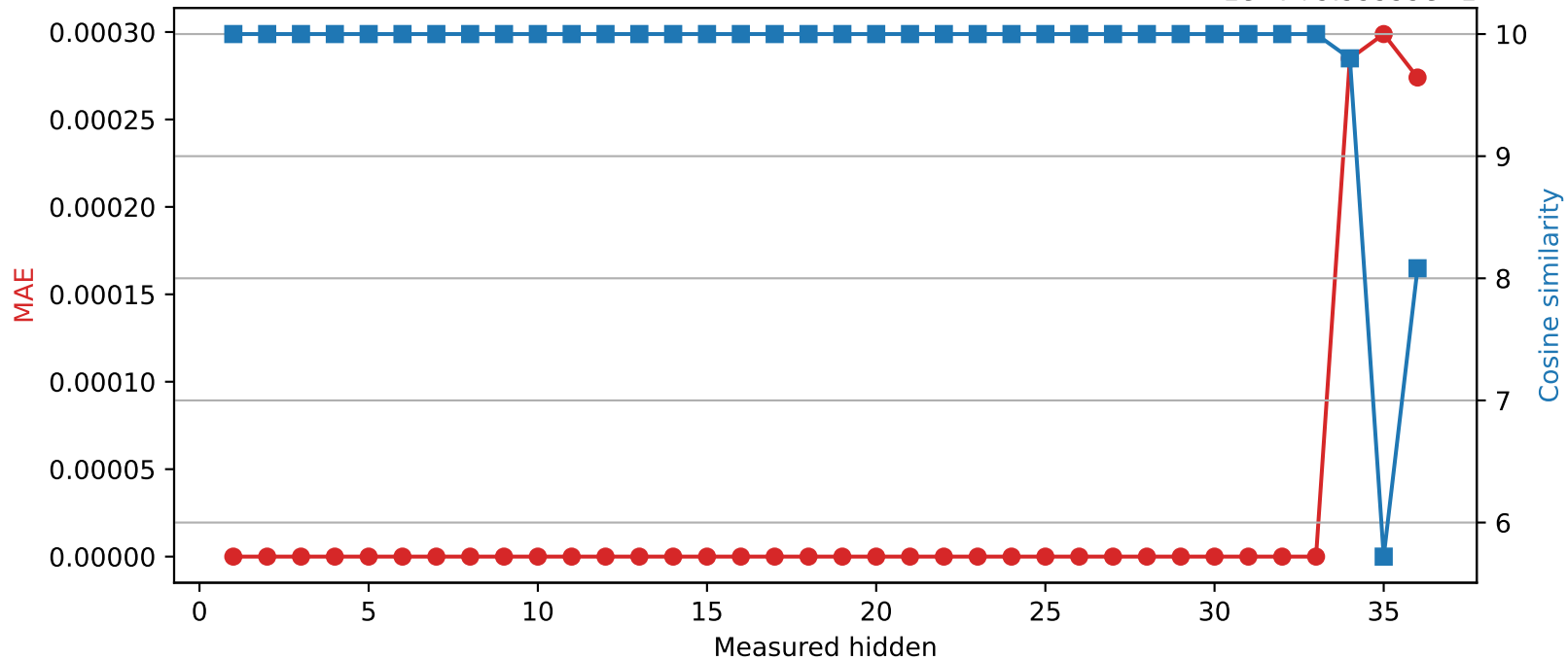
SmolLM3-3B | Quantized layer 33 | float64 \rightarrow int16 1e-7+9.99999e-1
