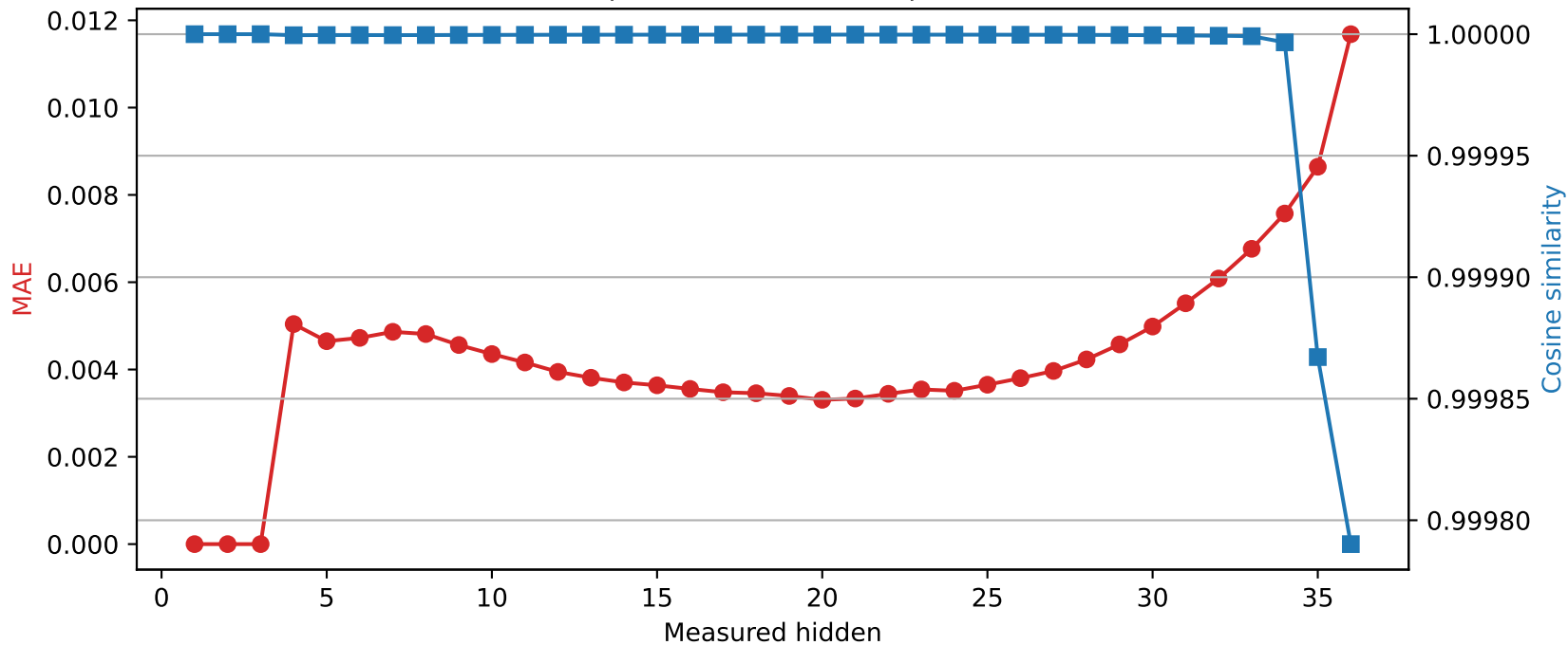
SmolLM3-3B | Quantized layer 3 | float16 \rightarrow int8
