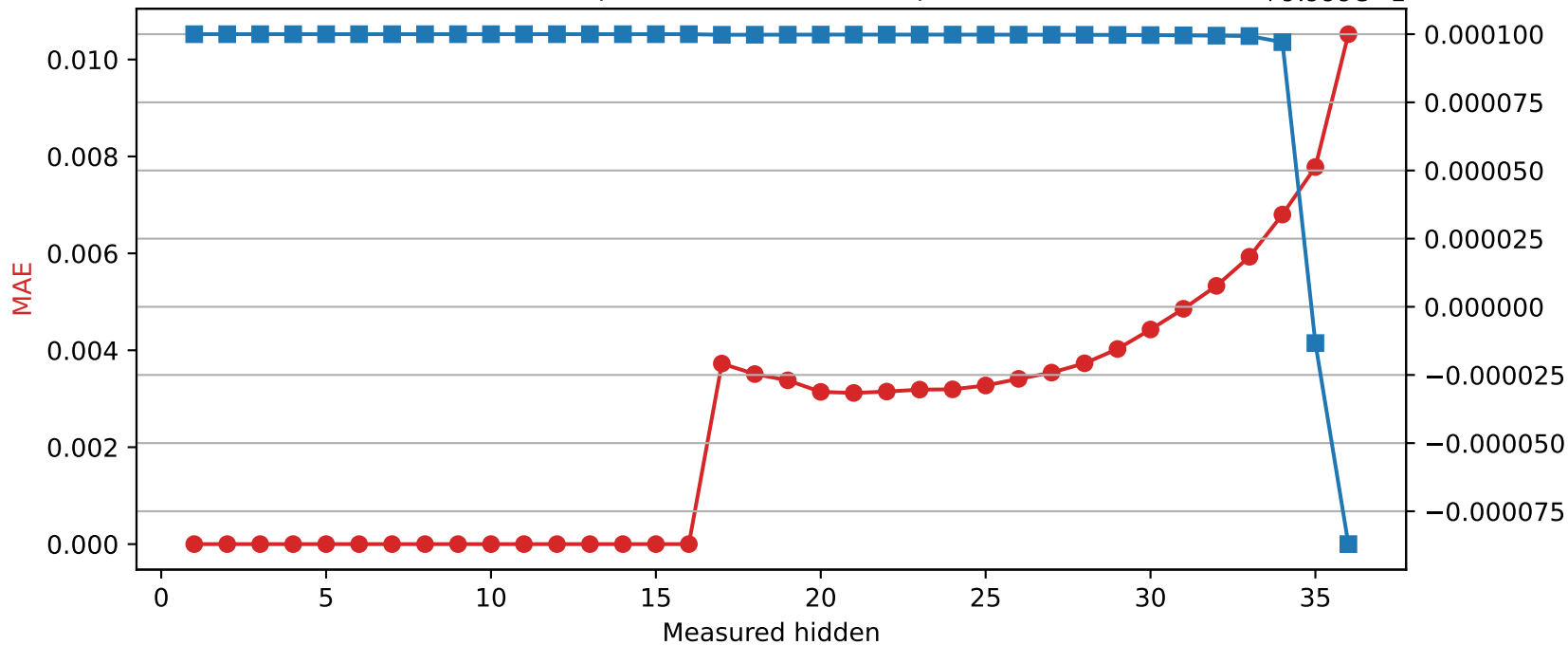
SmolLM3-3B | Quantized layer 16 | float16 → int8
