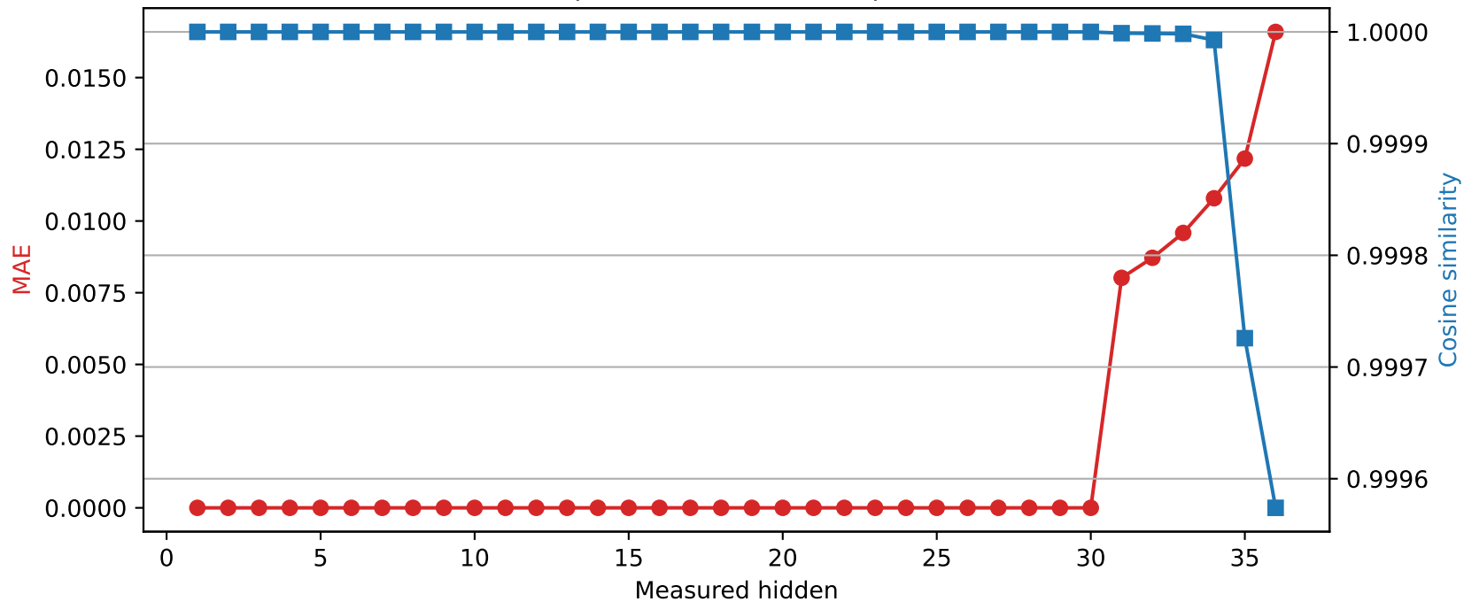
SmolLM3-3B | Quantized layer 30 | float16 → int8
