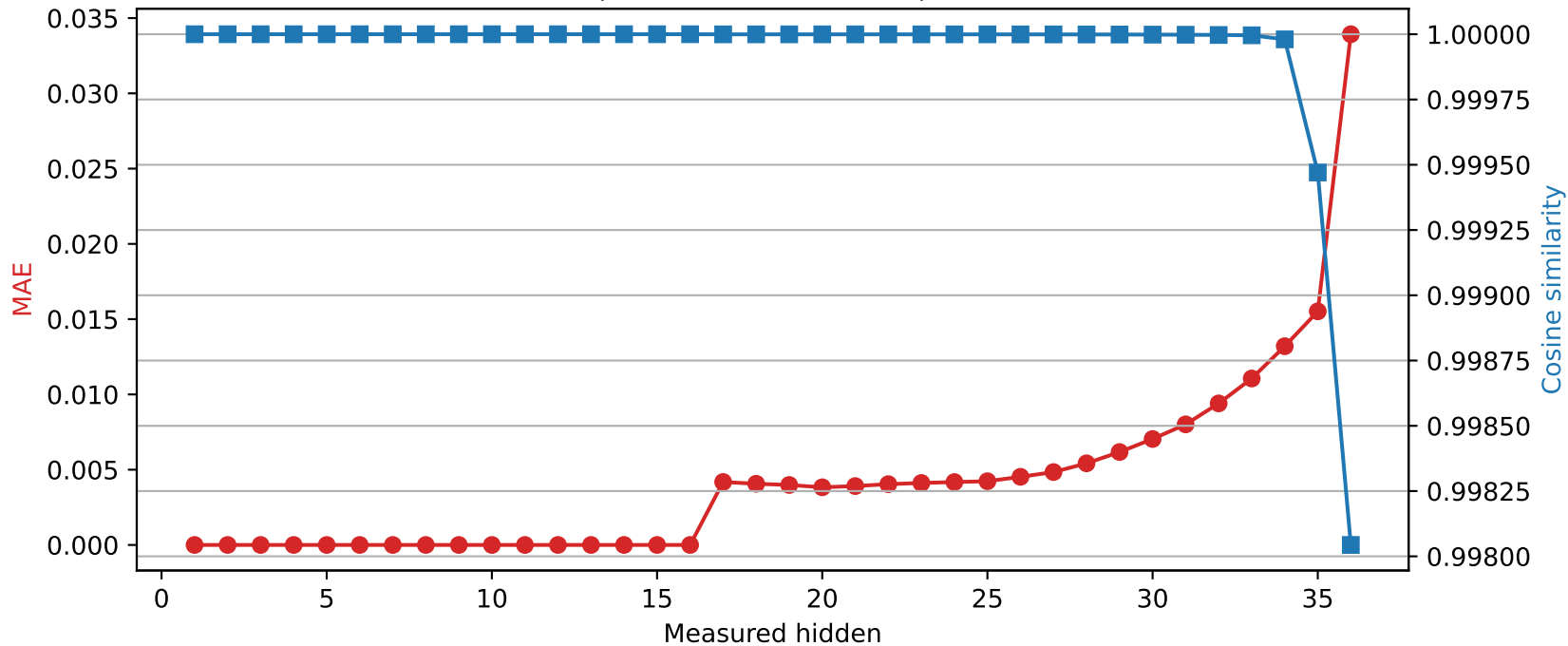
SmolLM3-3B | Quantized layer 16 | float16 \rightarrow int8
