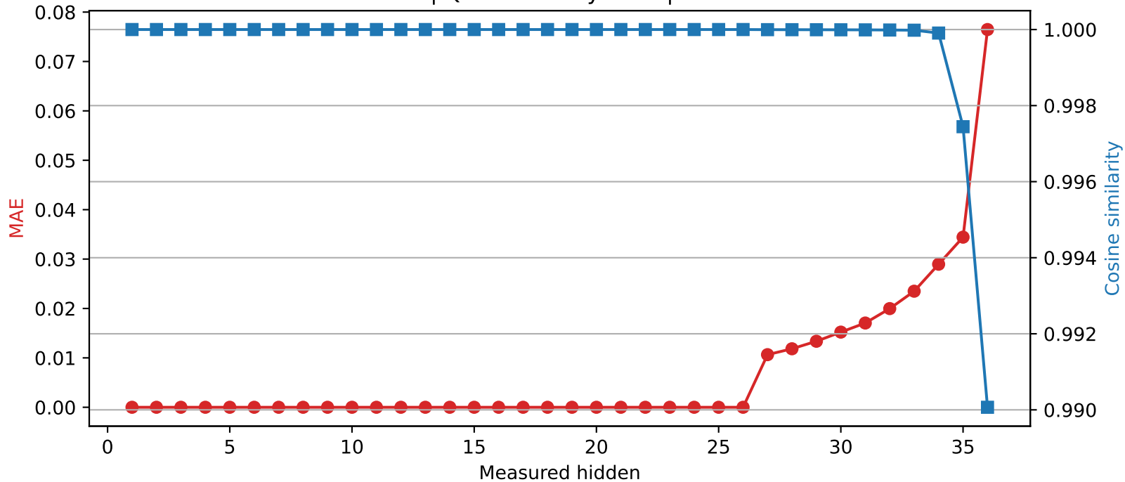
SmolLM3-3B | Quantized layer 26 | float16 → int8
