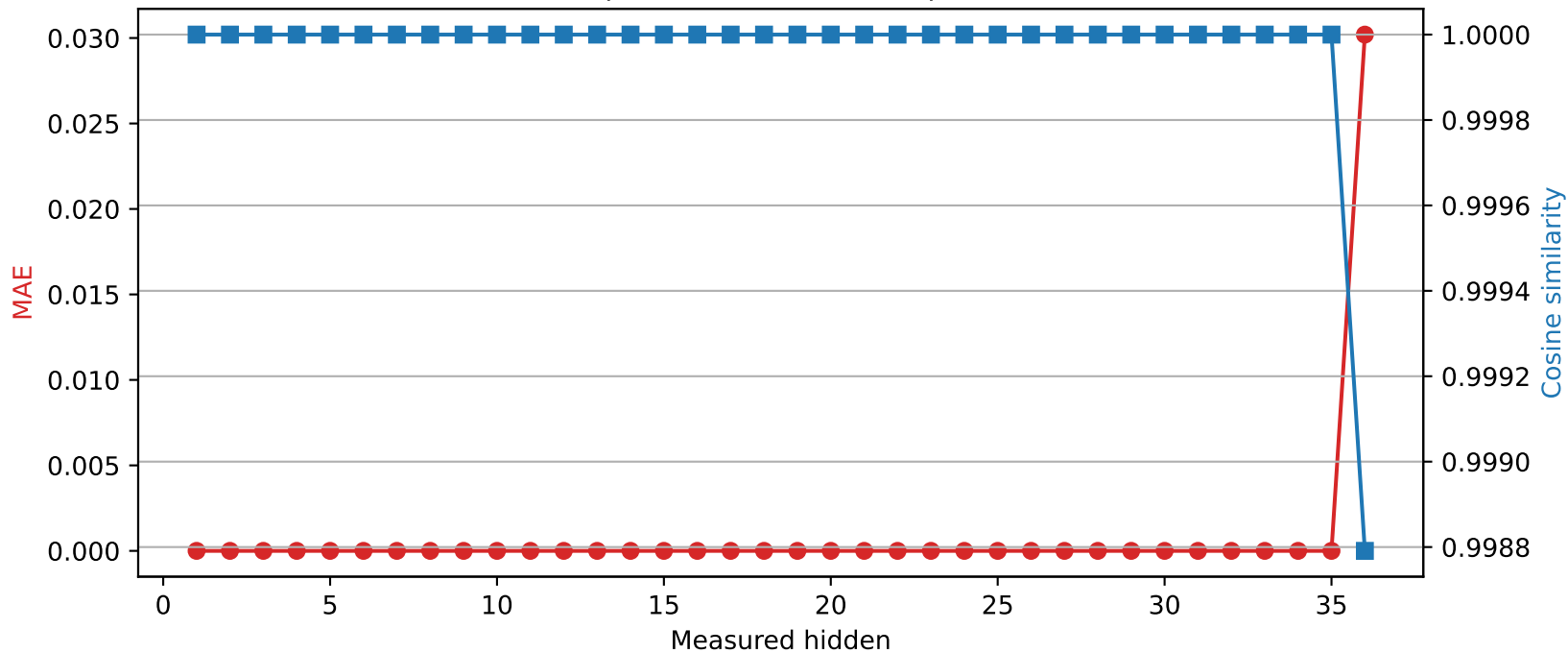
SmolLM3-3B | Quantized layer 35 | float16 \rightarrow int8
