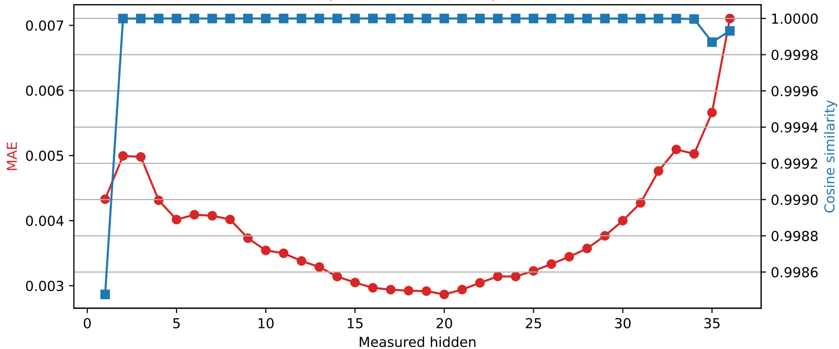
SmolLM3-3B | Quantized layer 0 | float16 → int8
