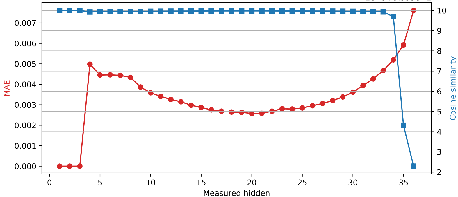
SmolLM3-3B | Quantized layer 3 | float16 → int8
