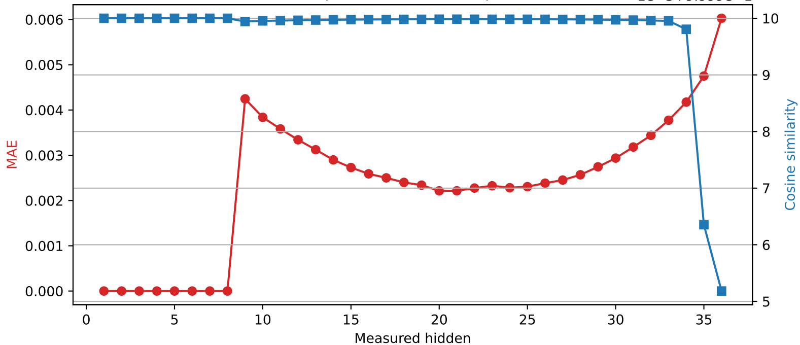
SmolLM3-3B | Quantized layer 8 | float16 → int8
