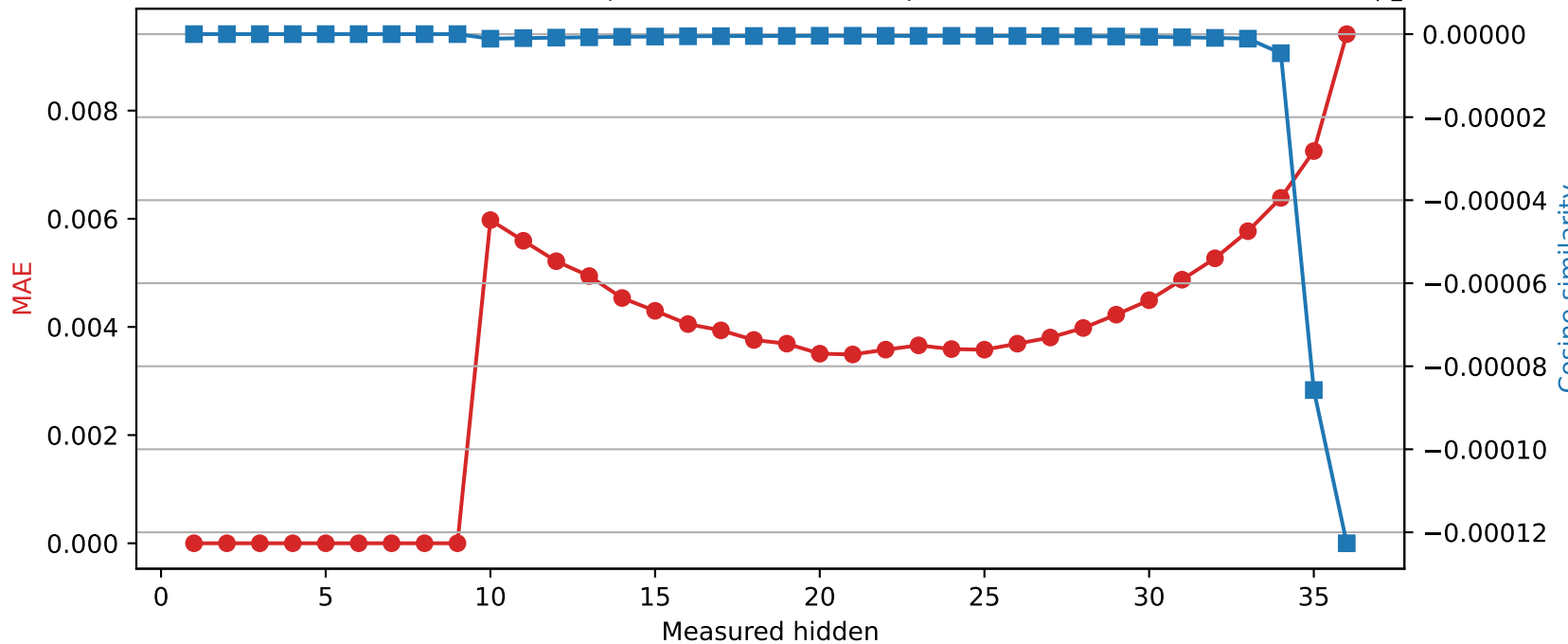
SmolLM3-3B | Quantized layer 9 | float16 → int8
