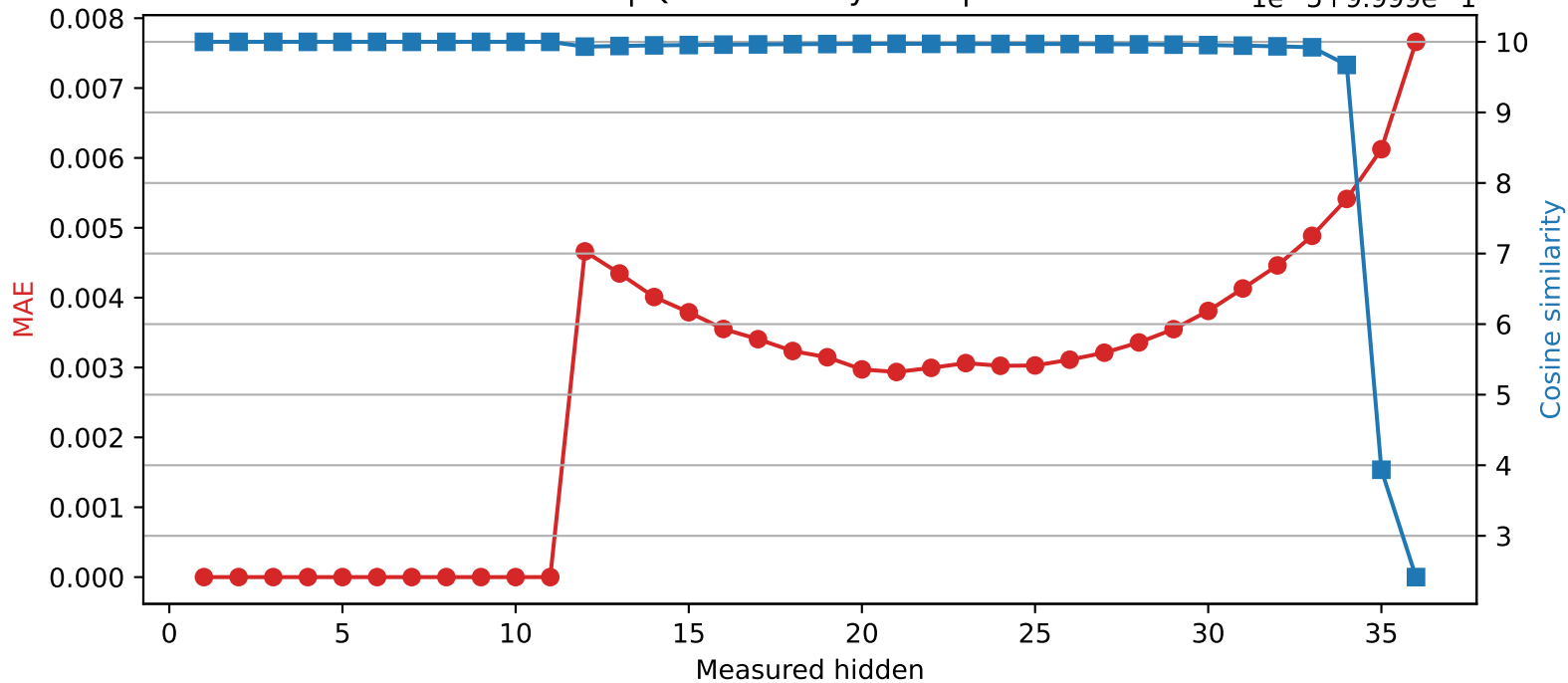
SmolLM3-3B | Quantized layer 11 | float16 → int8
