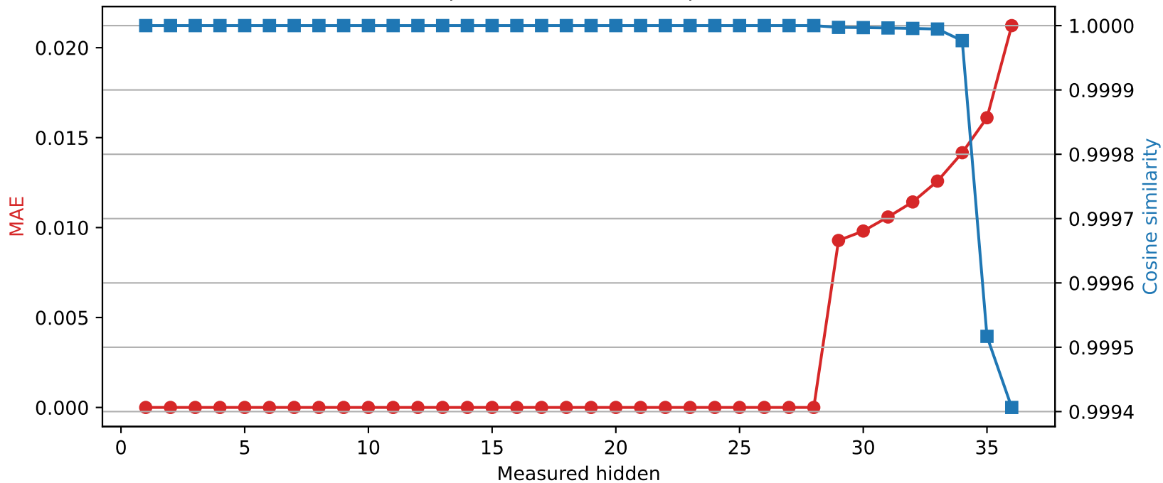
SmolLM3-3B | Quantized layer 28 | float16 → int8
