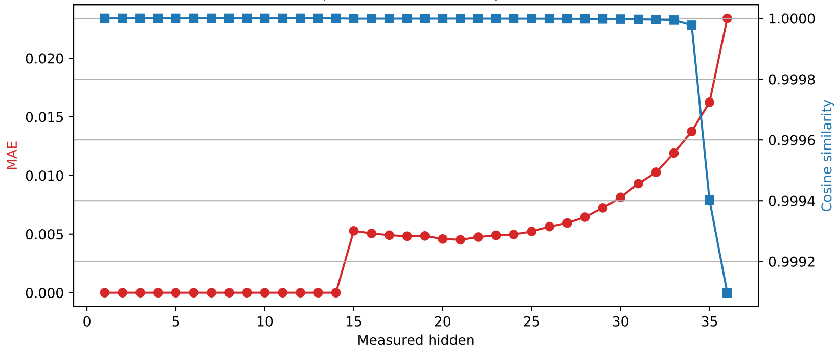
SmolLM3-3B | Quantized layer 14 | float16 \rightarrow int8
