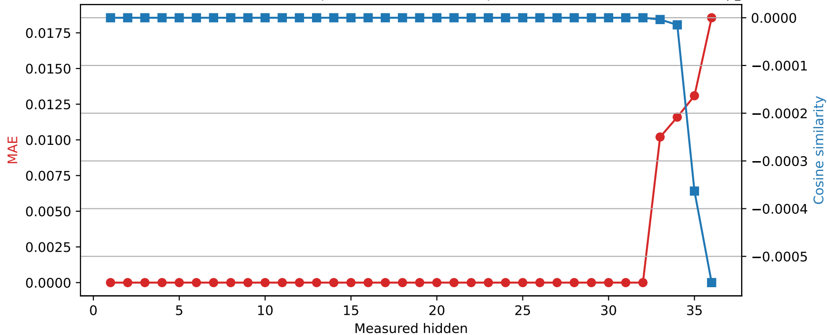
SmolLM3-3B | Quantized layer 32 | float16 → int8
