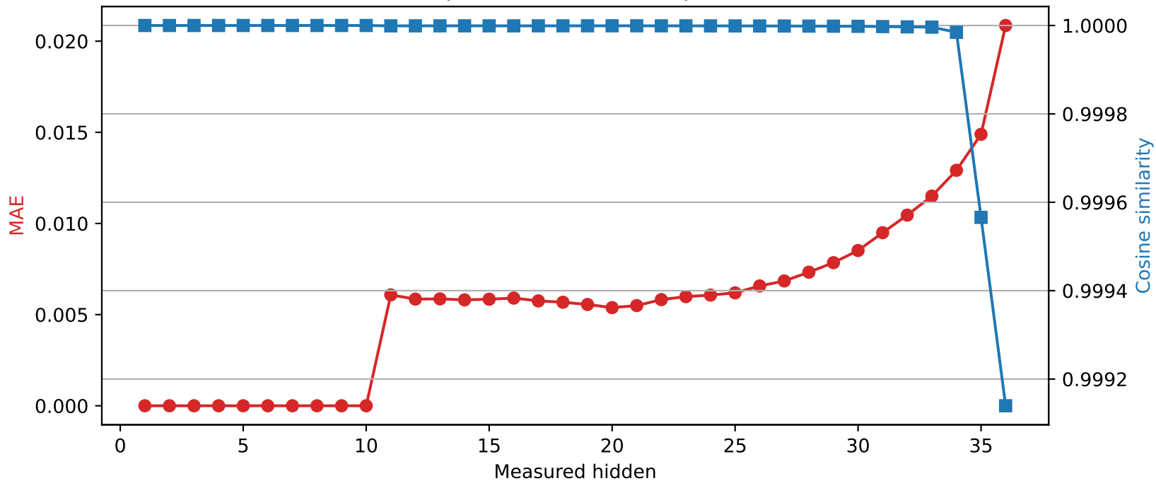
SmolLM3-3B | Quantized layer 10 | float16 \rightarrow int8
