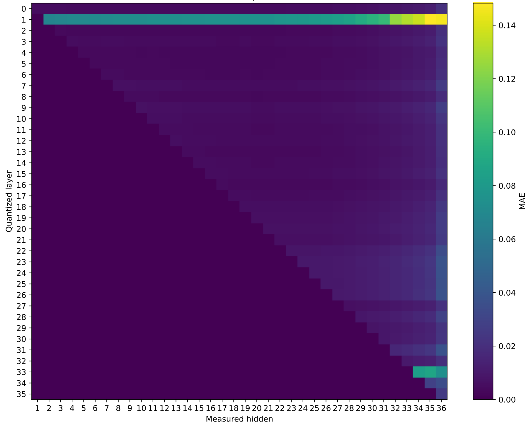
Model: SmolLM3-3B | float32 → int8
