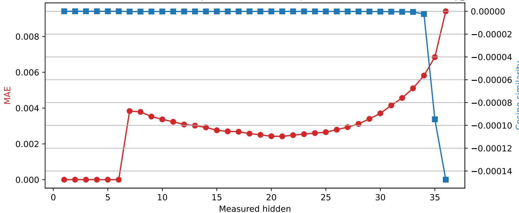
SmolLM3-3B | Quantized layer 6 | float32 → int8
