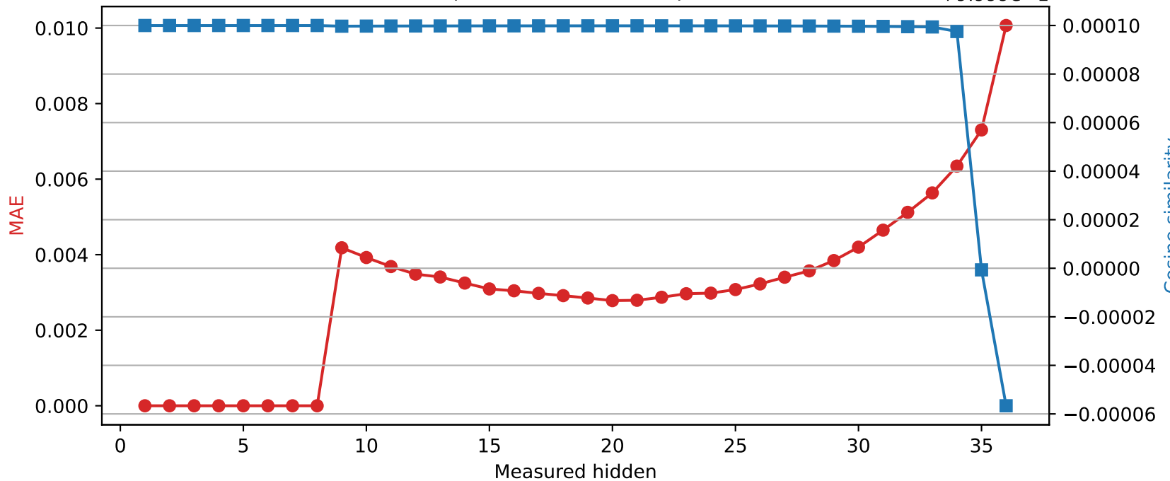
SmolLM3-3B | Quantized layer 8 | float32 → int8
