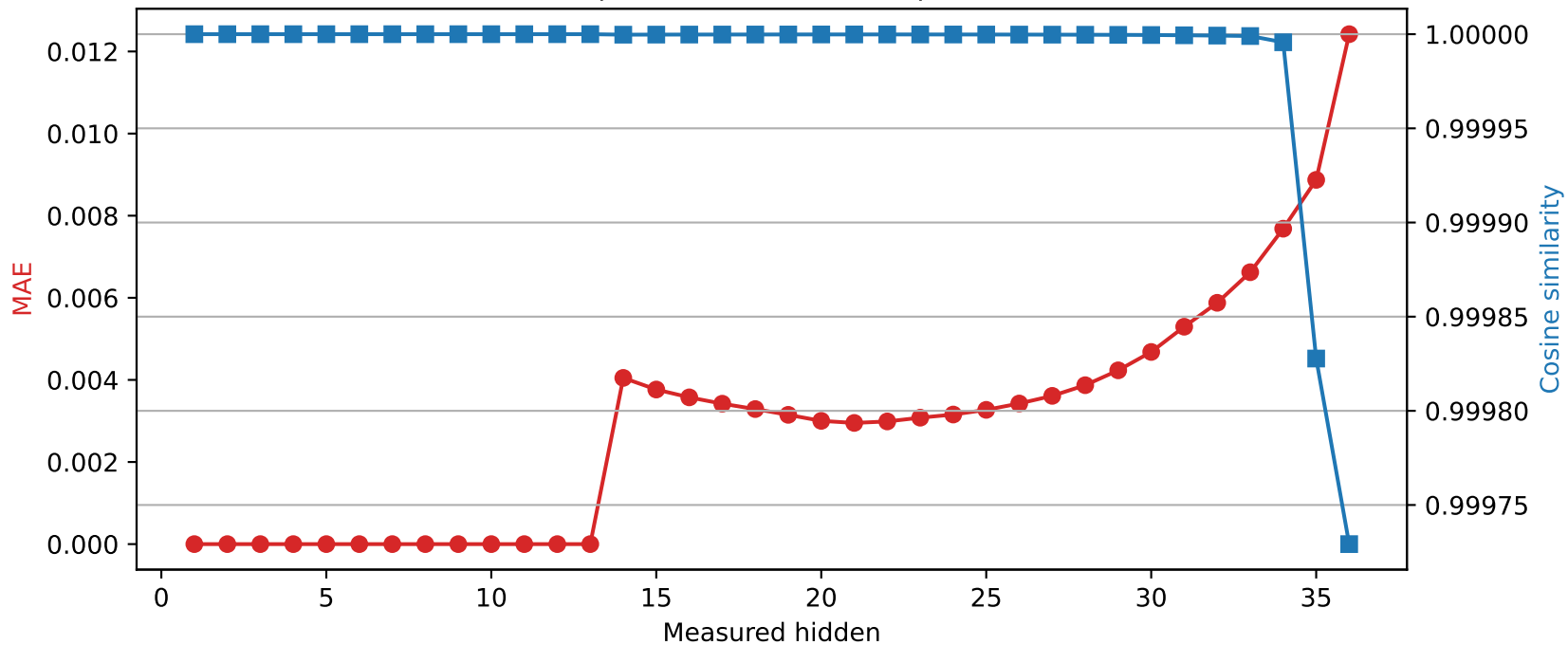
SmolLM3-3B | Quantized layer 13 | float32 → int8
