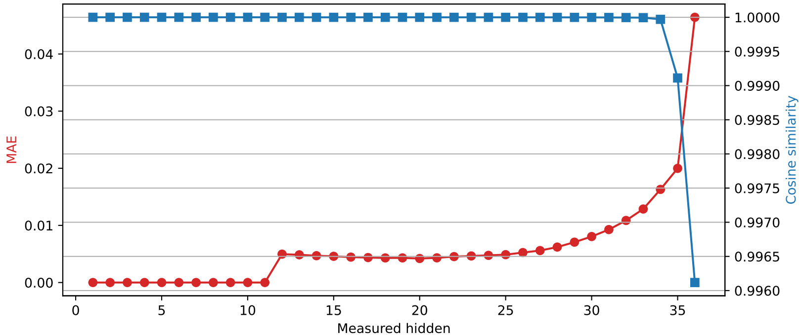
SmolLM3-3B | Quantized layer 11 | float32 → int8
