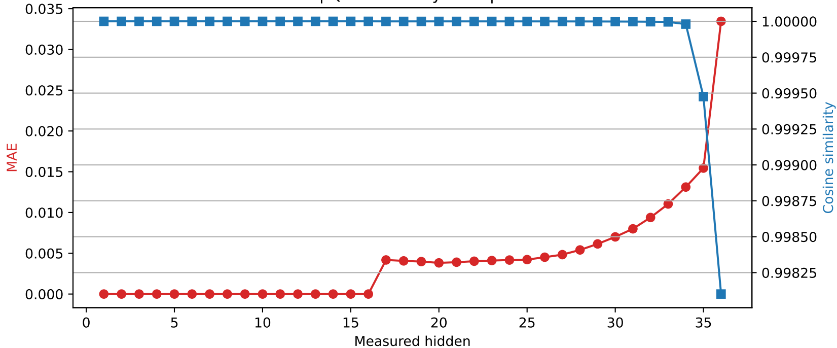
SmolLM3-3B | Quantized layer 16 | float32 → int8
