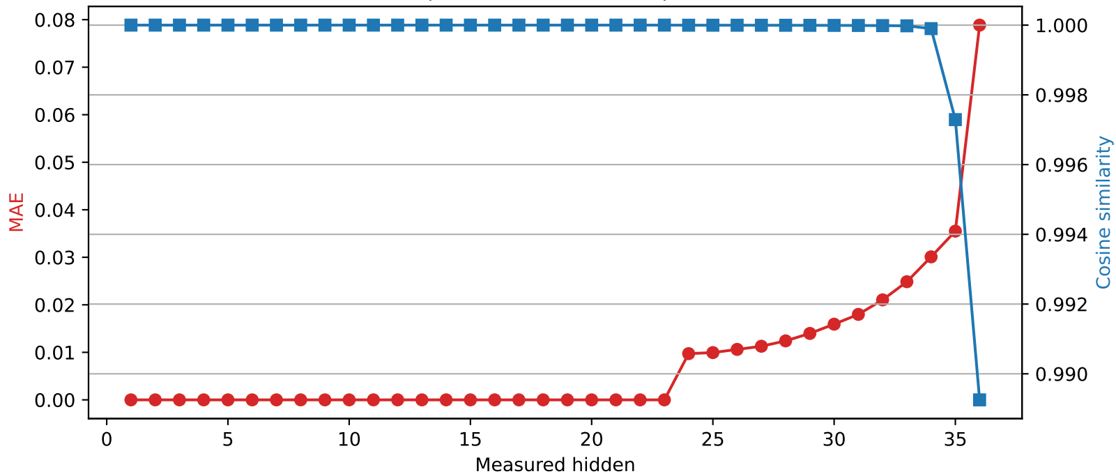
SmolLM3-3B | Quantized layer 23 | float32 \rightarrow int8
