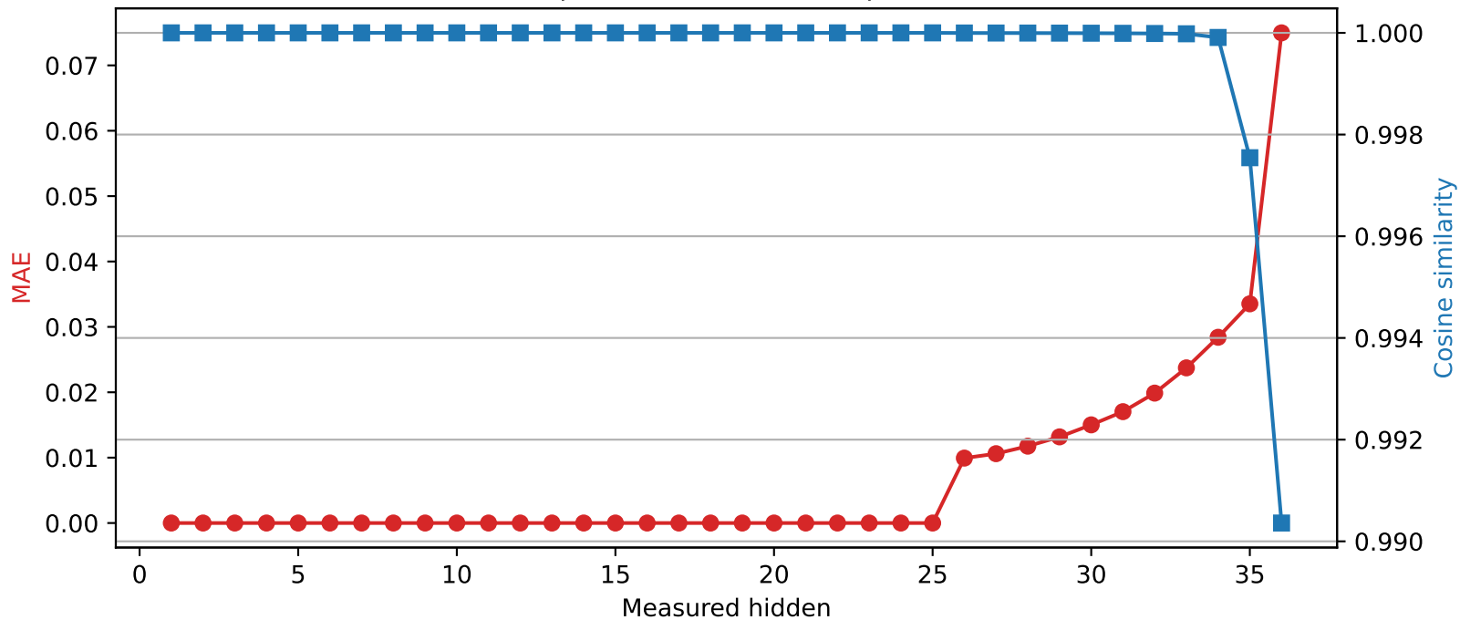
SmolLM3-3B | Quantized layer 25 | float32 → int8
