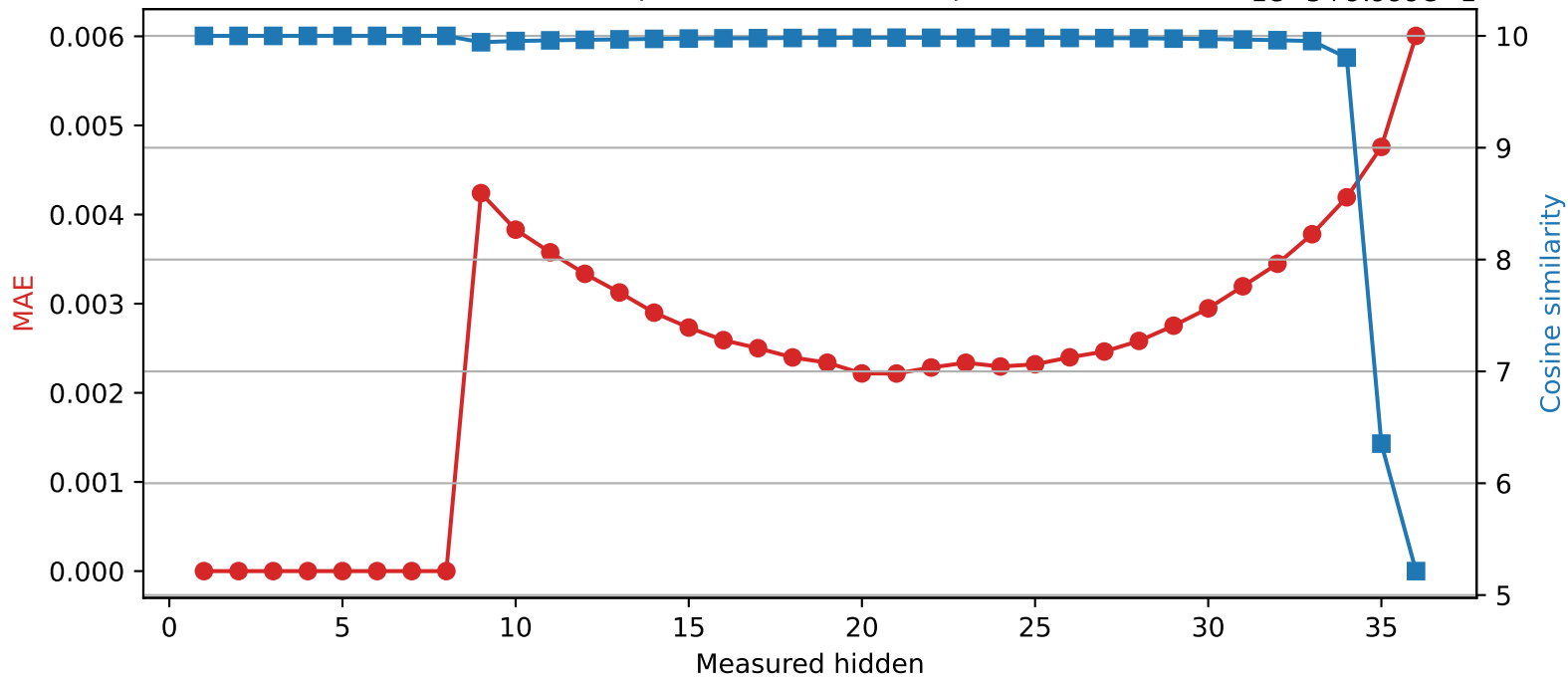
SmolLM3-3B | Quantized layer 8 | float32 → int8
