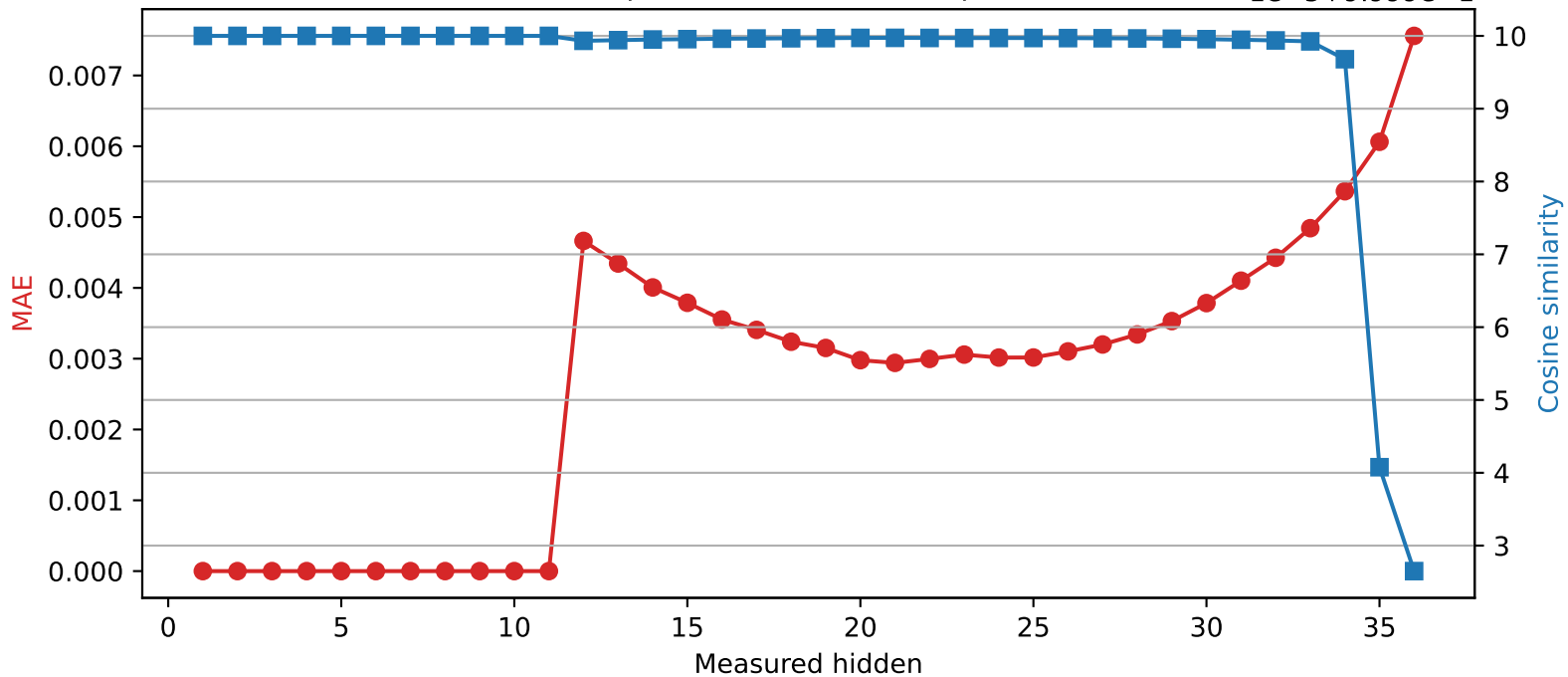
SmolLM3-3B | Quantized layer 11 | float32 → int8
