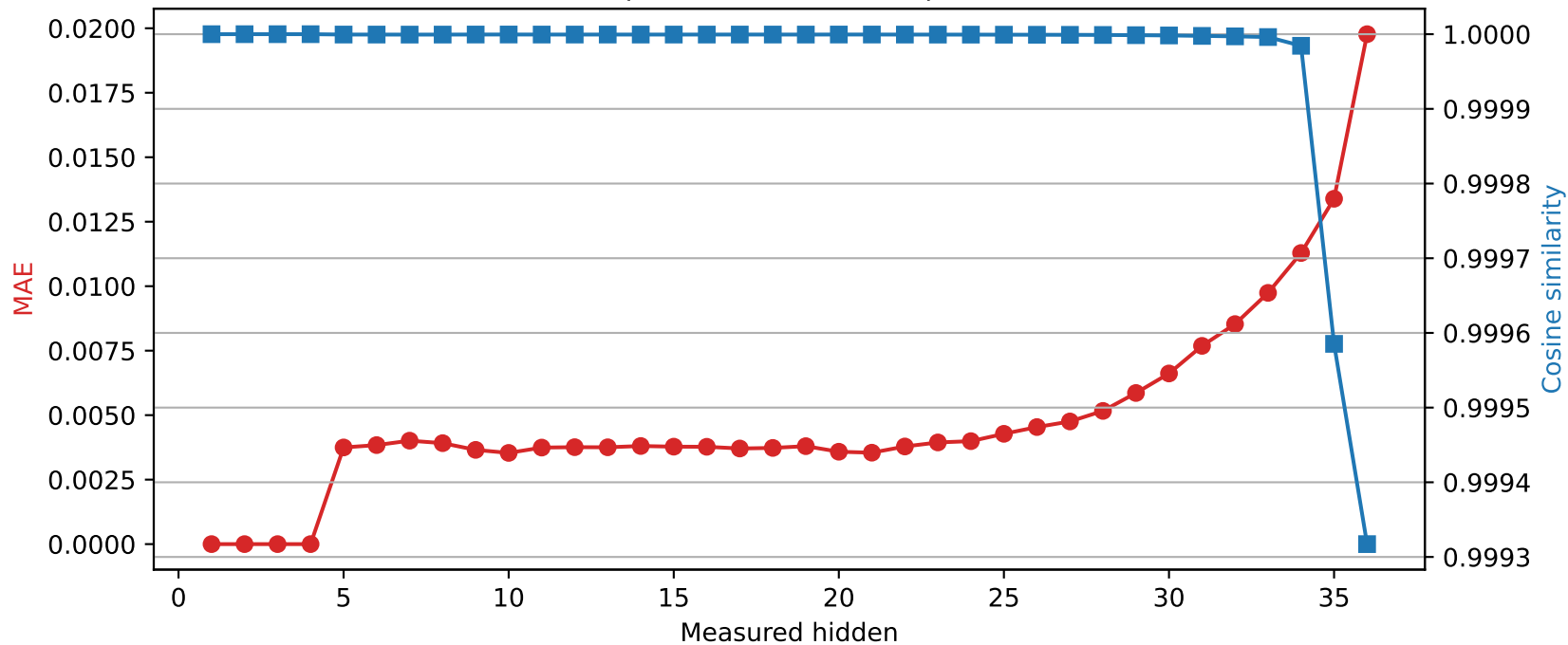
SmolLM3-3B | Quantized layer 4 | float32 \rightarrow int8
