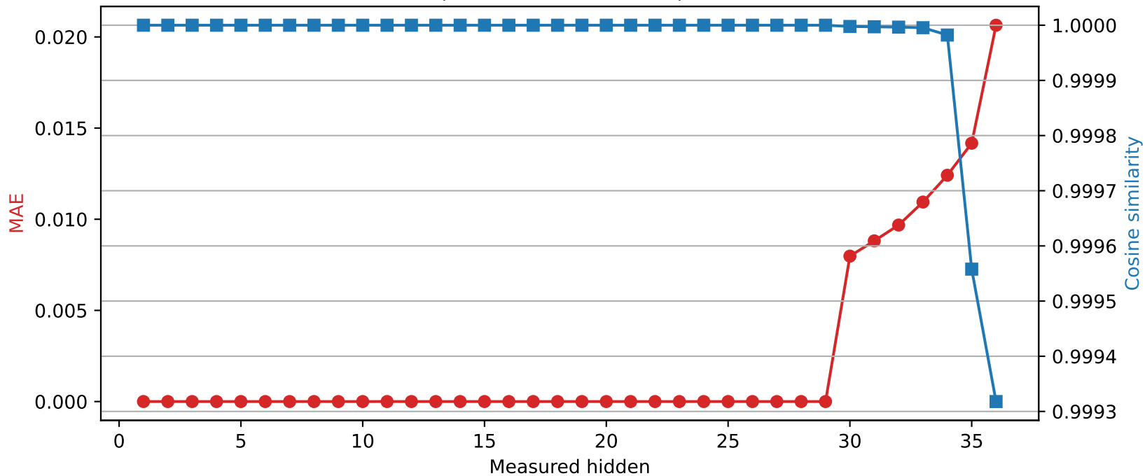
SmolLM3-3B | Quantized layer 29 | float32 → int8
