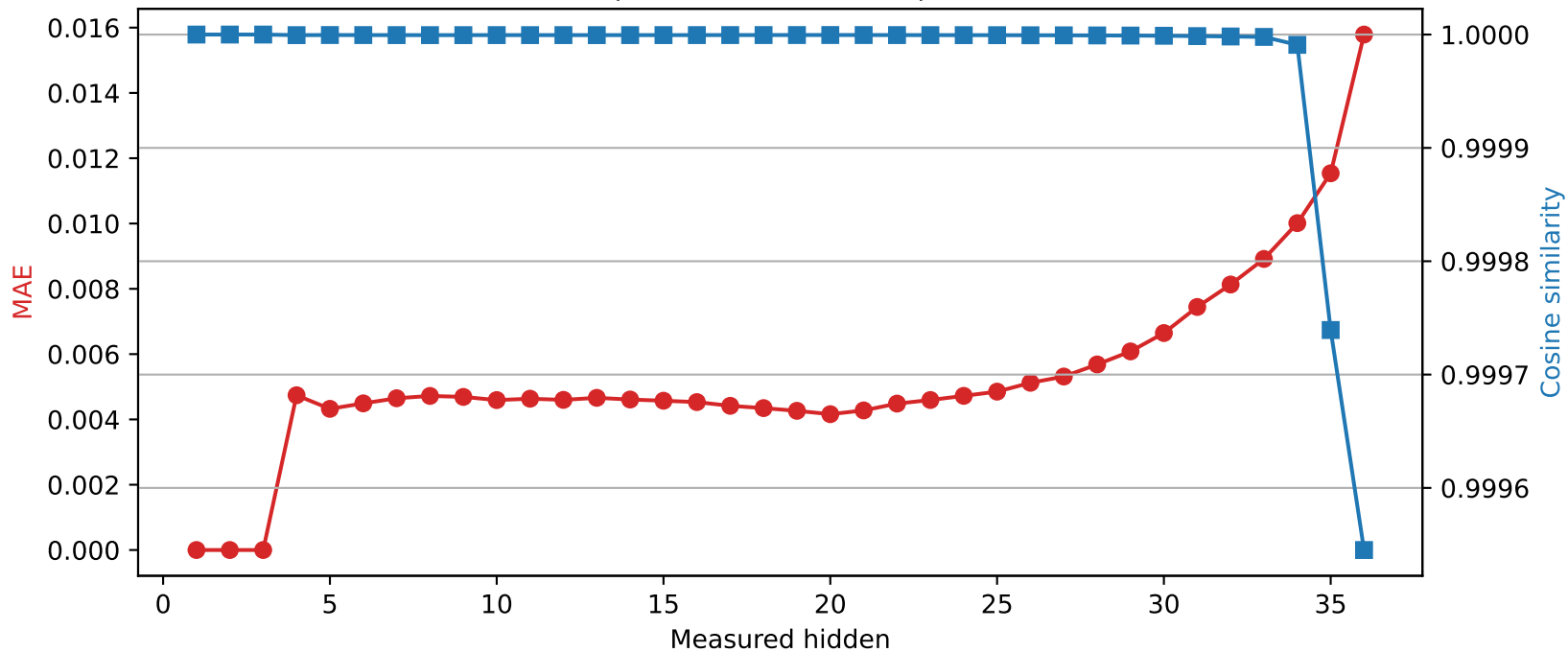
SmolLM3-3B | Quantized layer 3 | float32 → int8
