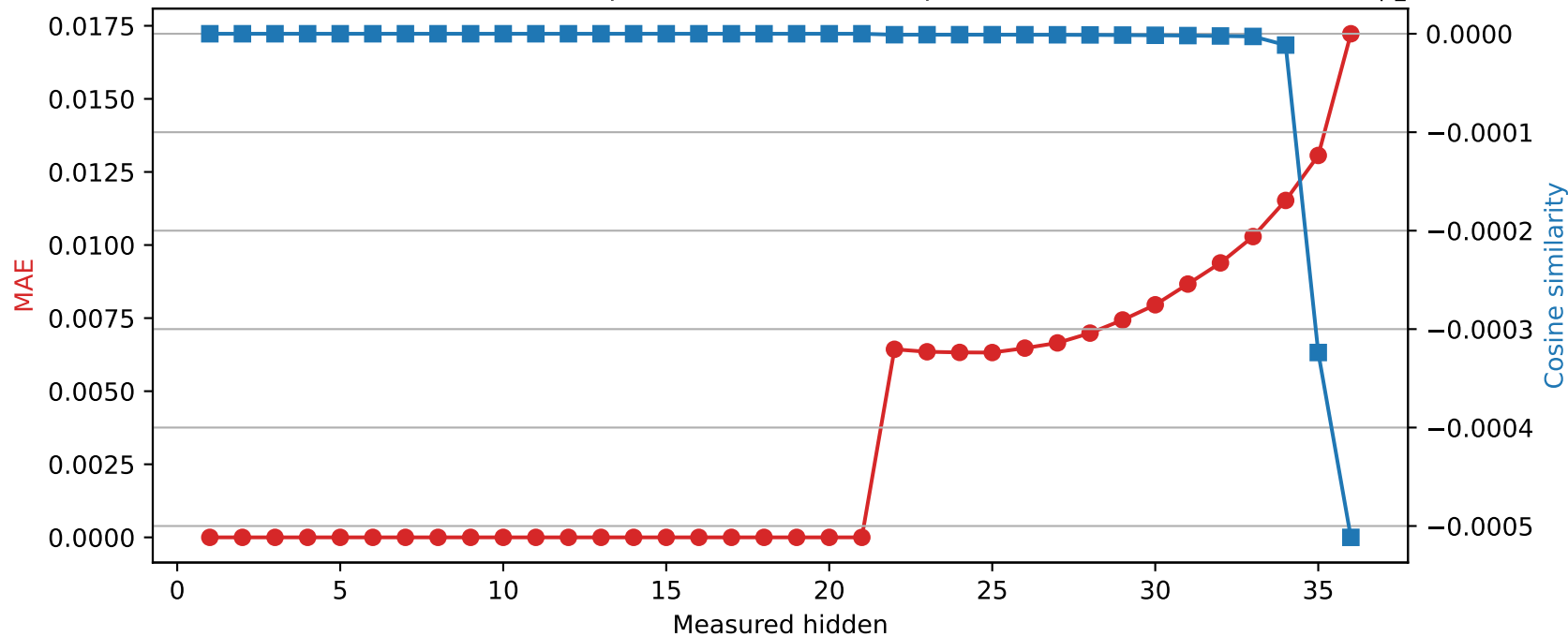
SmolLM3-3B | Quantized layer 21 | float32 → int8
