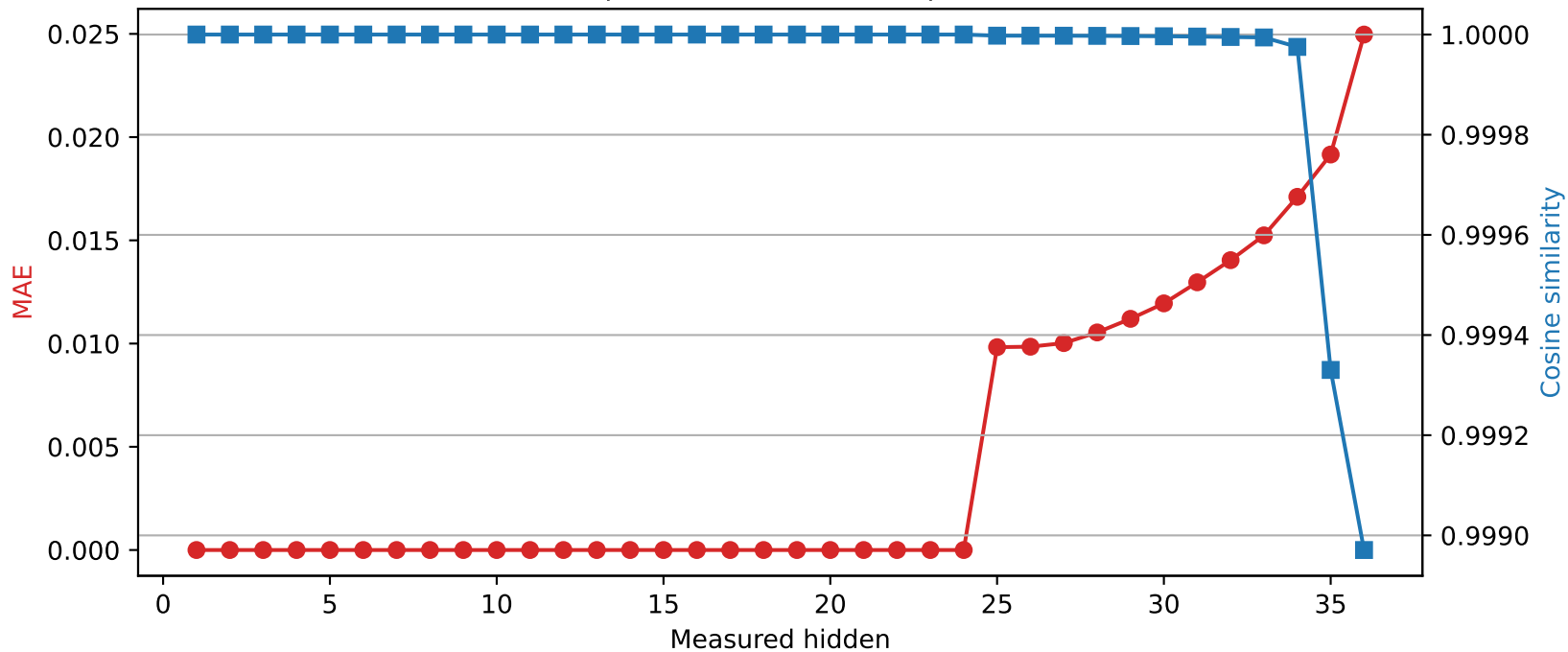
SmolLM3-3B | Quantized layer 24 | float32 → int8
