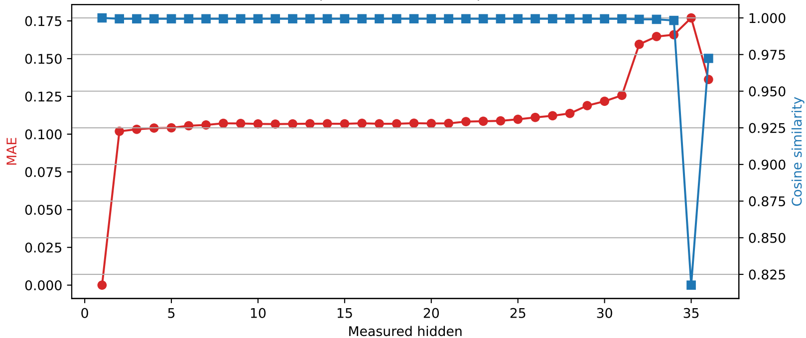
SmolLM3-3B | Quantized layer 1 | float64 → int8
