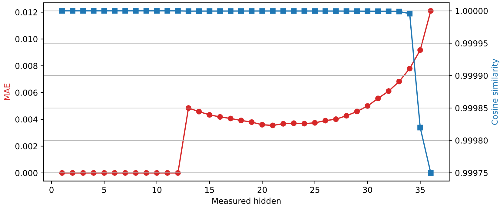
SmolLM3-3B | Quantized layer 12 | float64 → int8
