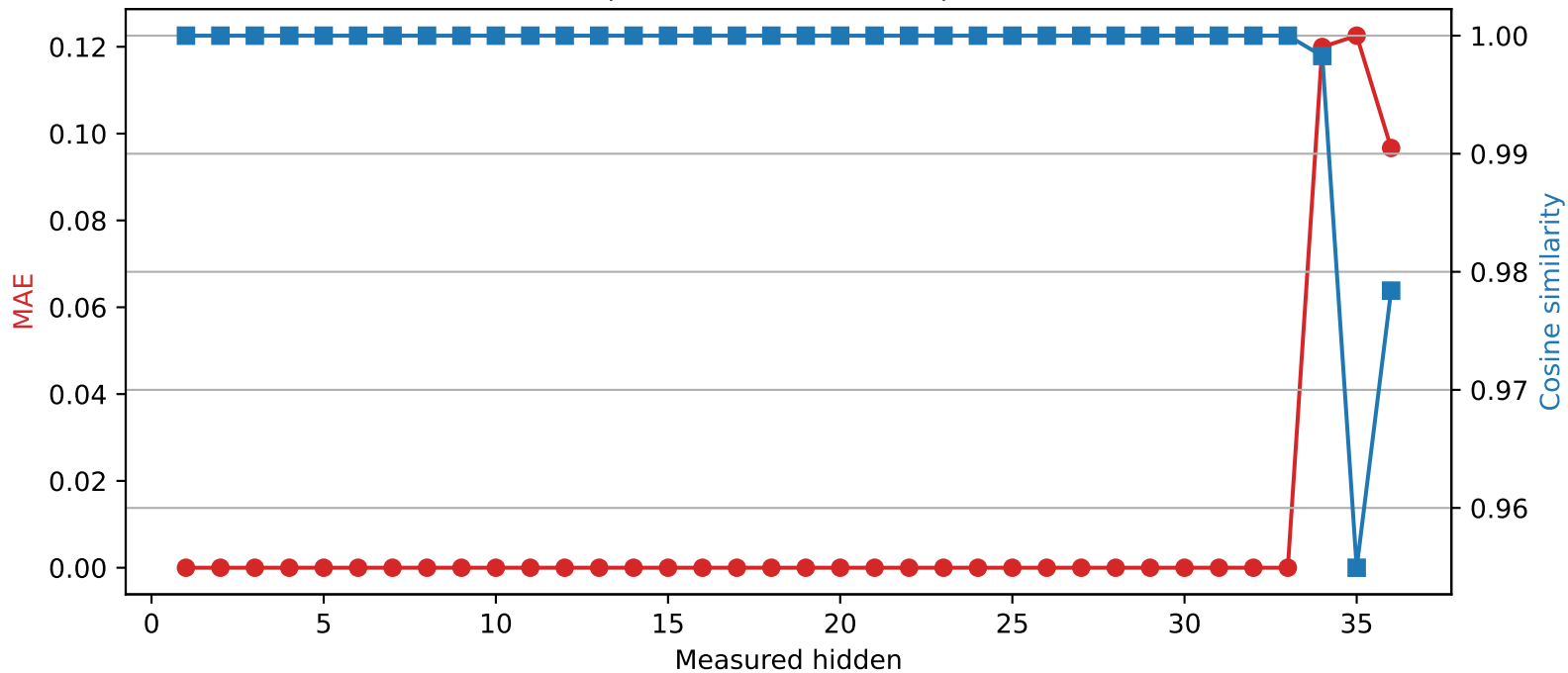
SmolLM3-3B | Quantized layer 33 | float64 → int8
