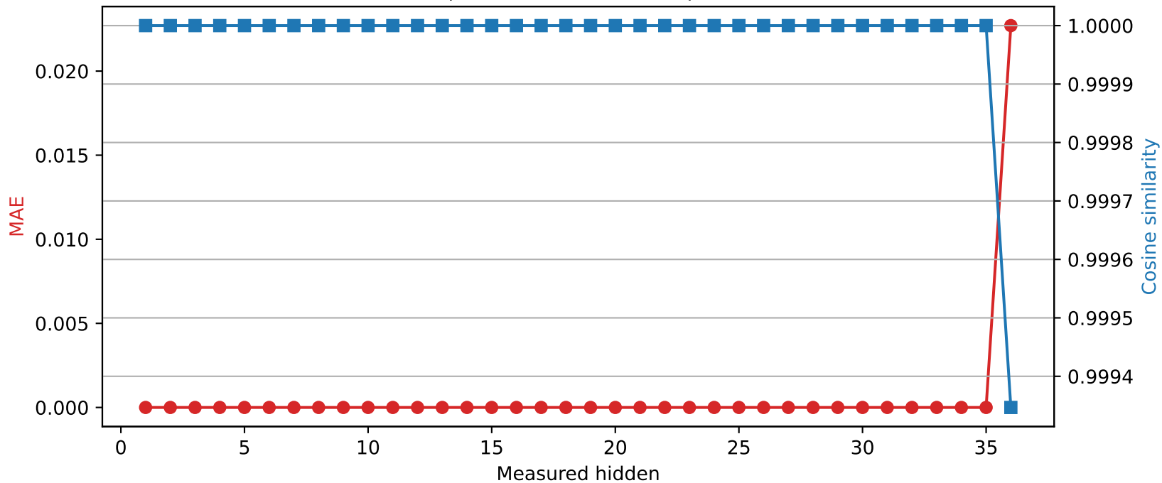
SmolLM3-3B | Quantized layer 35 | float64 → int8
