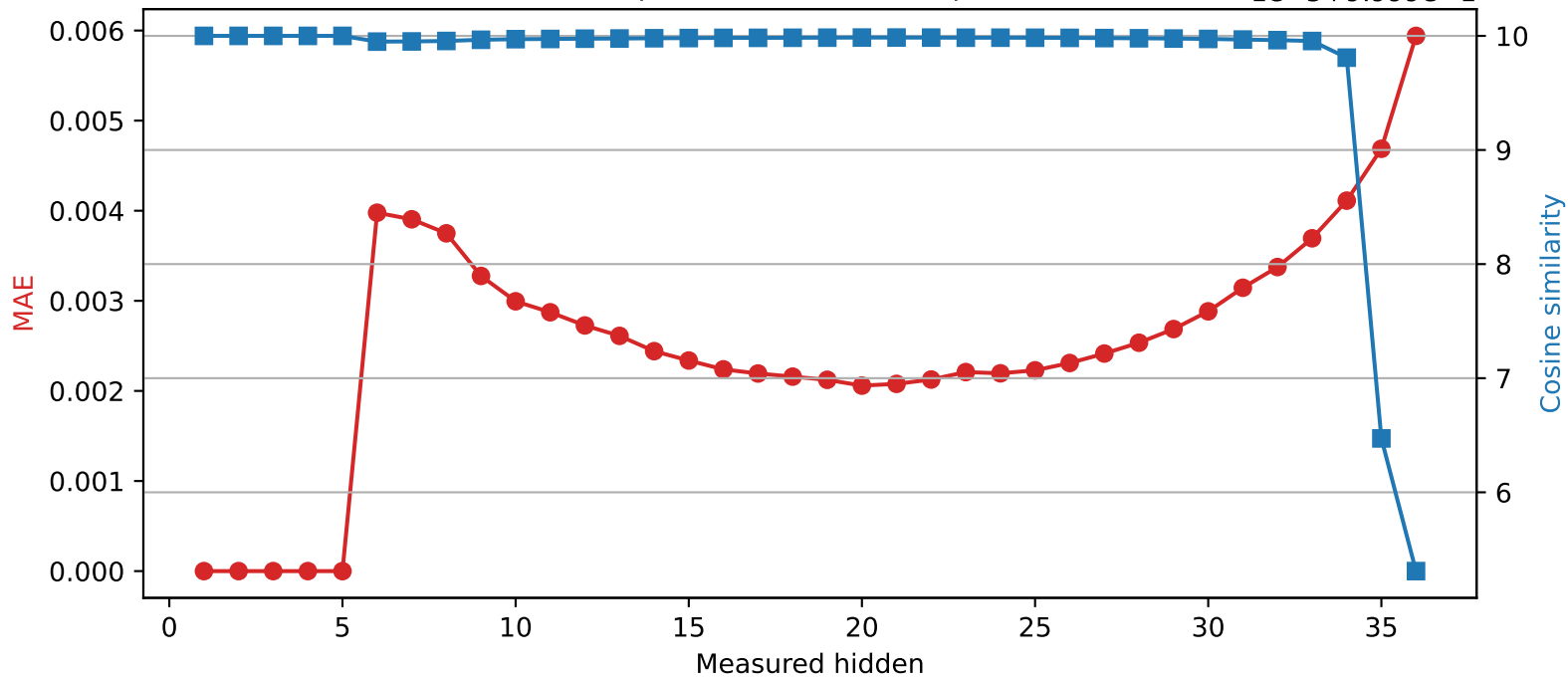
SmolLM3-3B | Quantized layer 5 | float64 → int8
