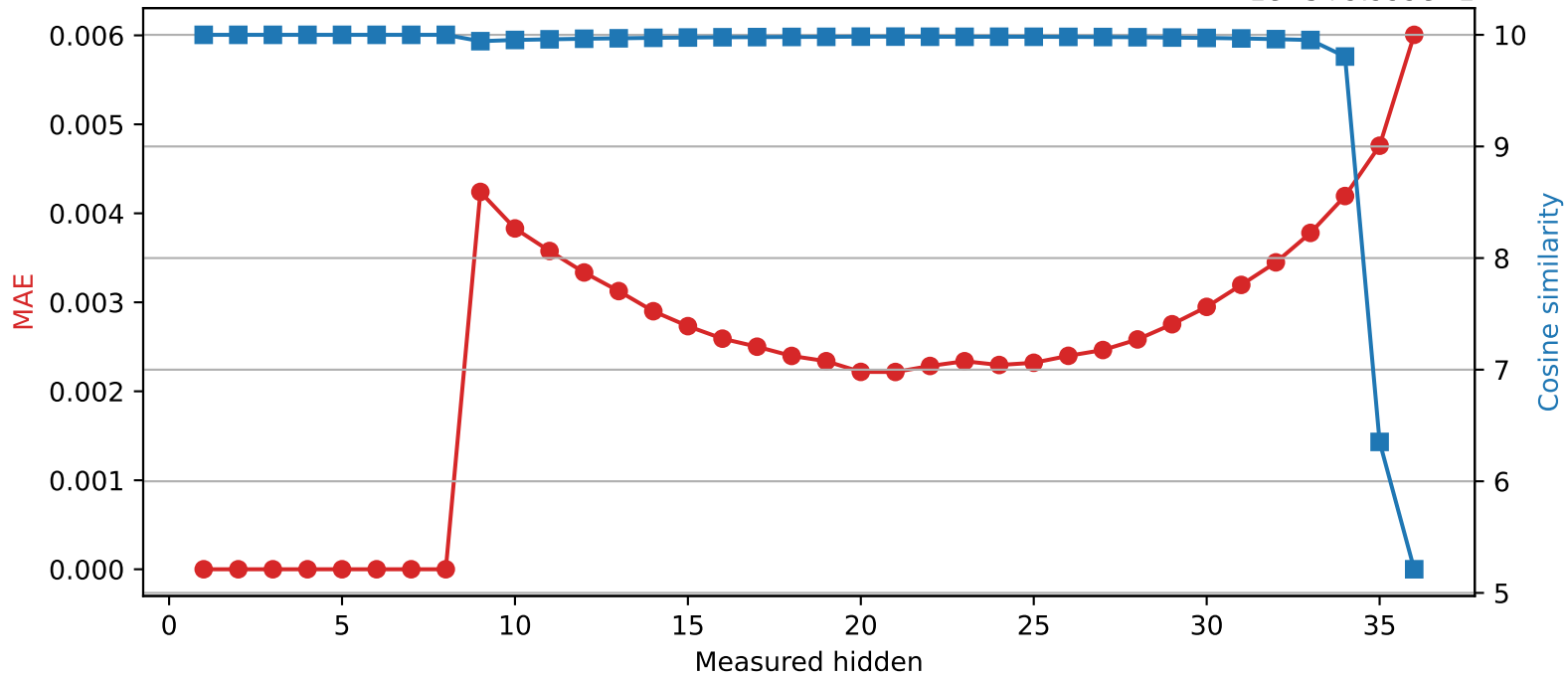
SmolLM3-3B | Quantized layer 8 | float64 → int8
