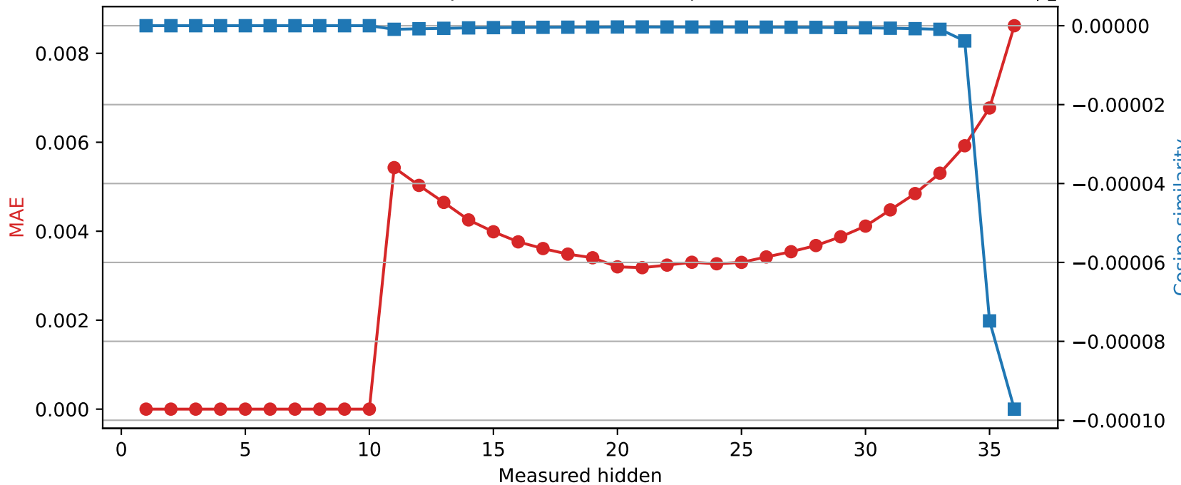
SmolLM3-3B | Quantized layer 10 | float64 → int8
